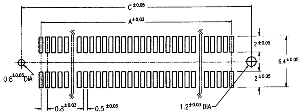
RECOMMENDED P.W. BOARD LAYOUT
