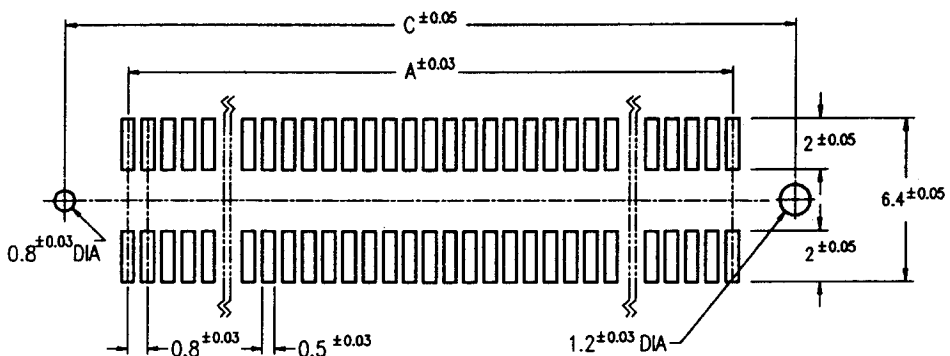
RECOMMENDED P.W. BOARD LAYOUT
